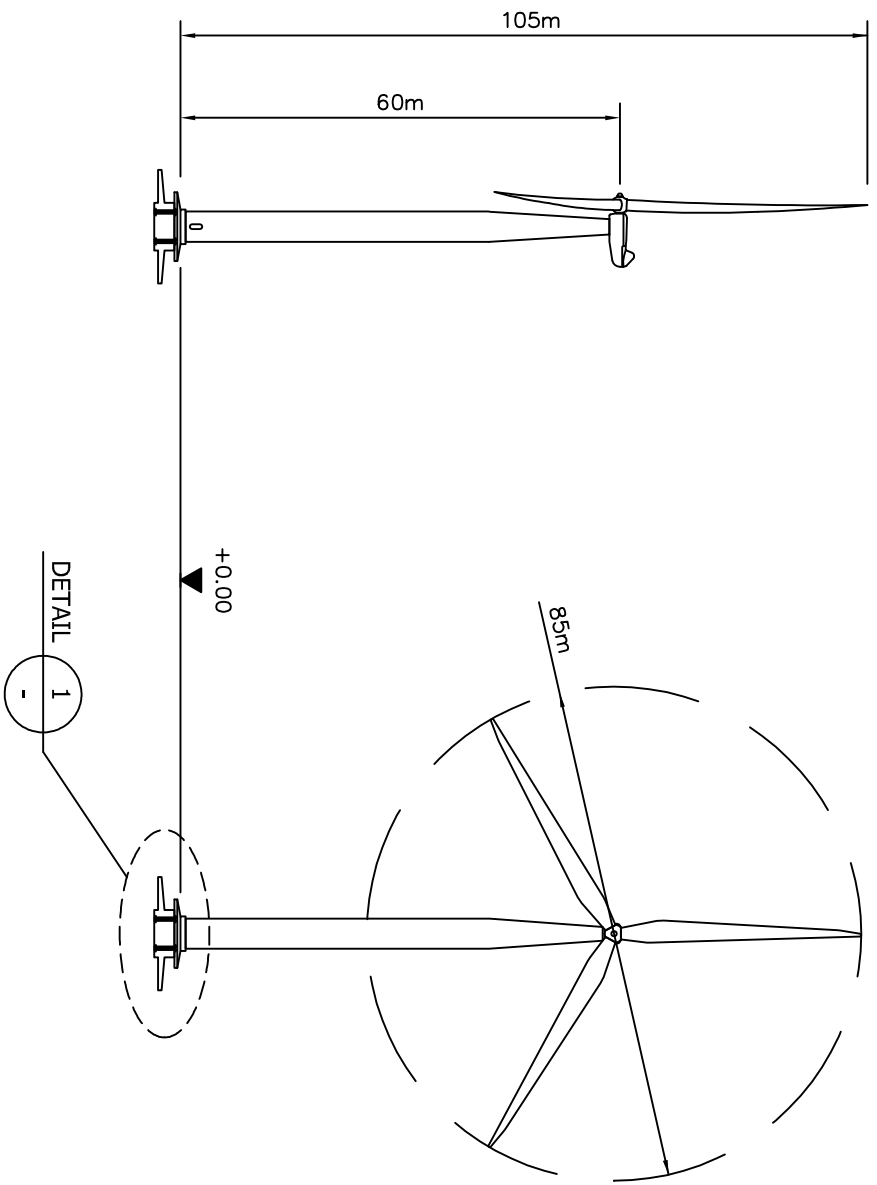
Proposed Hemsby Turbine Detail Scale 1:500 @ A1
